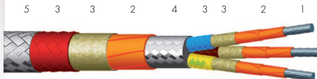
THS 1400 M
